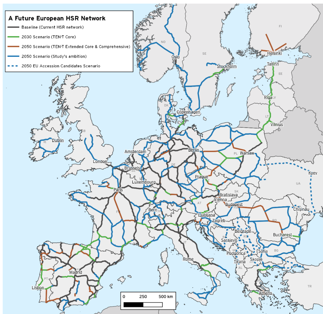
Figure 5: HSR network, all scenarios 32
