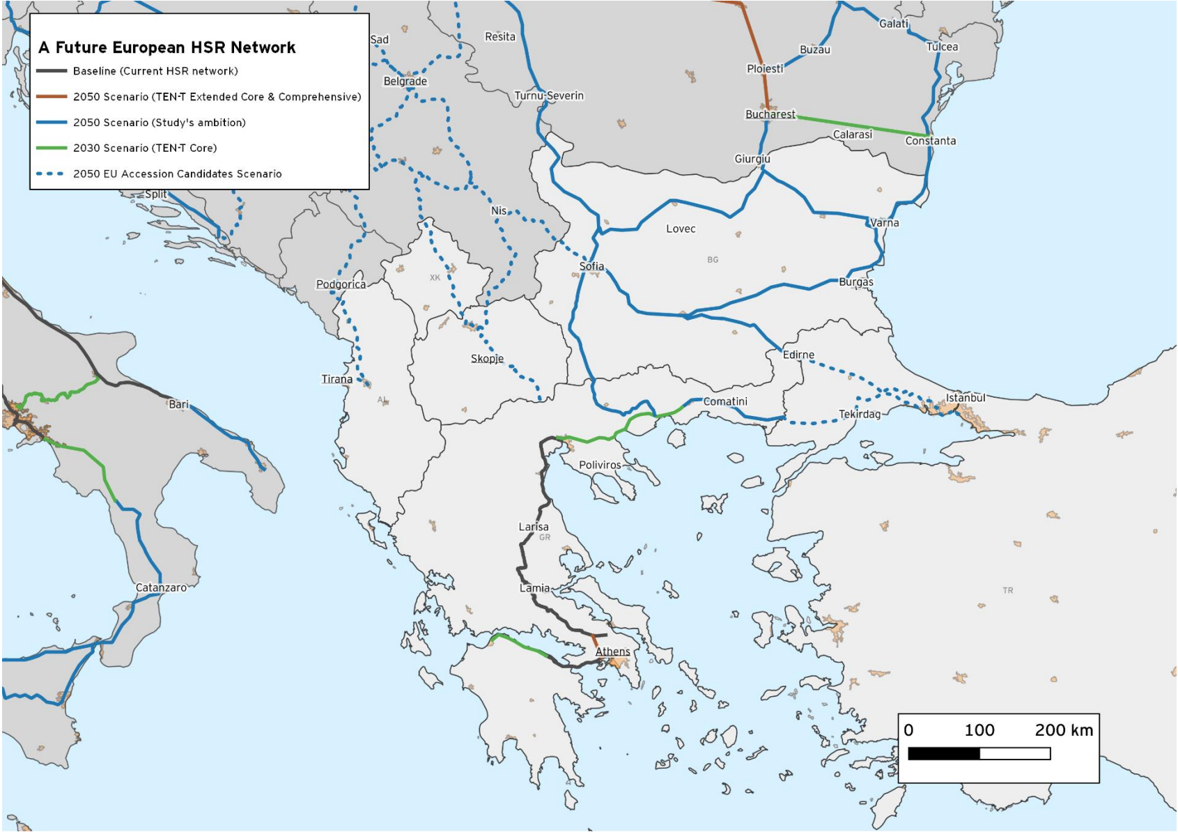
Figure 22: HSR network - Macedonia, Bulgaria, Albania, Greece and Turkey
