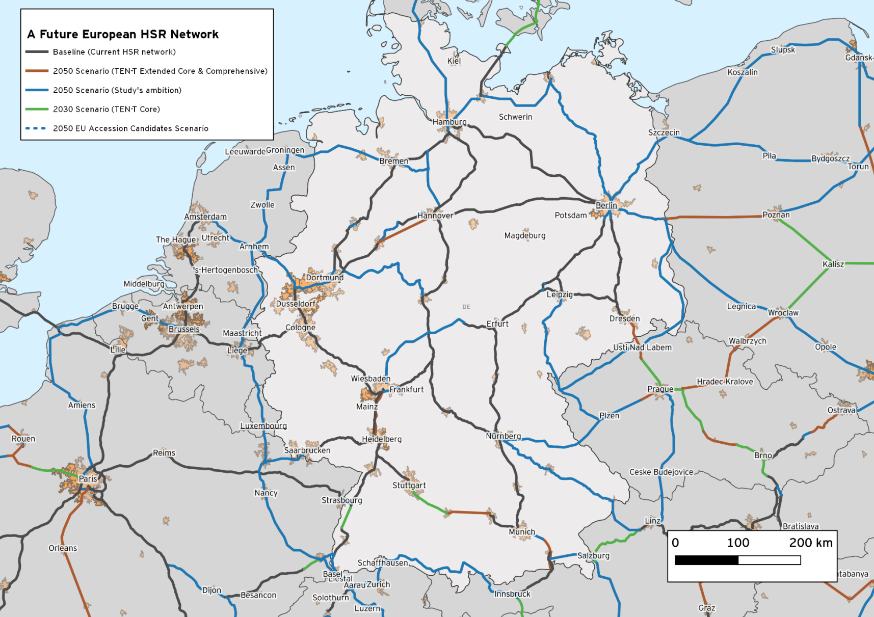
Figure 35: HSR network - Germany
