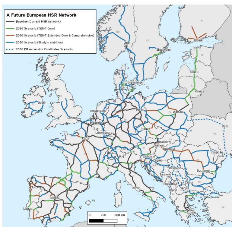
Figure 6: The Future HSR Network under different scenarios
