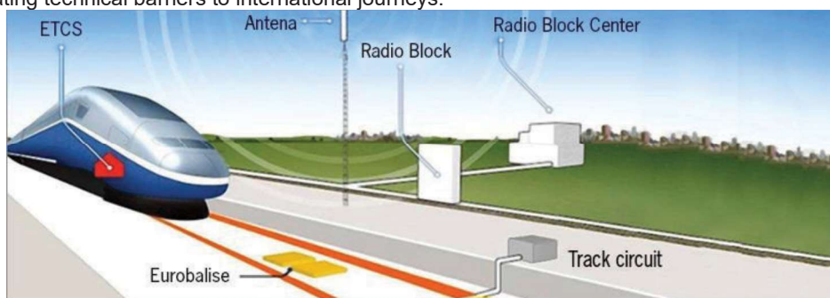
ERTMS components
