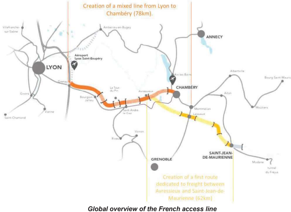
Global overview of the French access line
