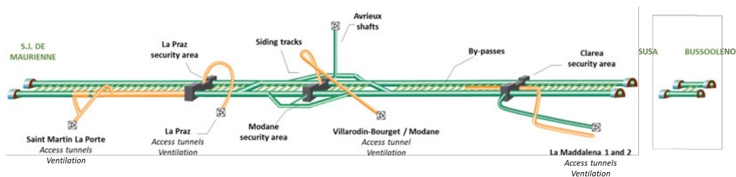
The Mont Cenis base tunnel of the NLTL (Orange components are completed)
